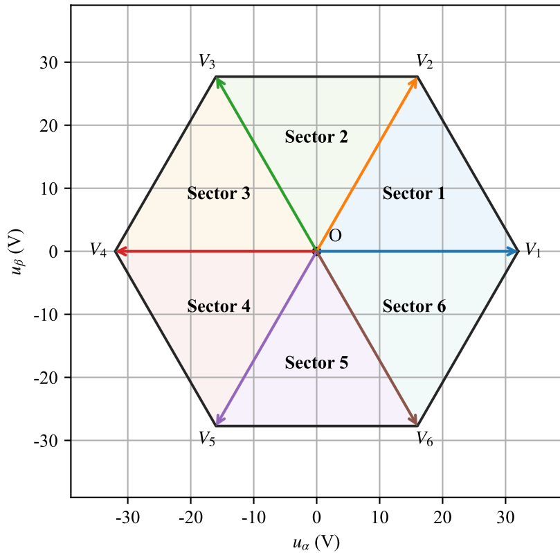
SVPWM sector distribution, U_{dc} = 48\text{ V}
